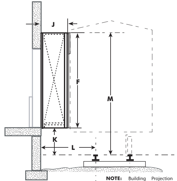
NOTE: Building Projection Past Dock Face Wall - Consult Factory
